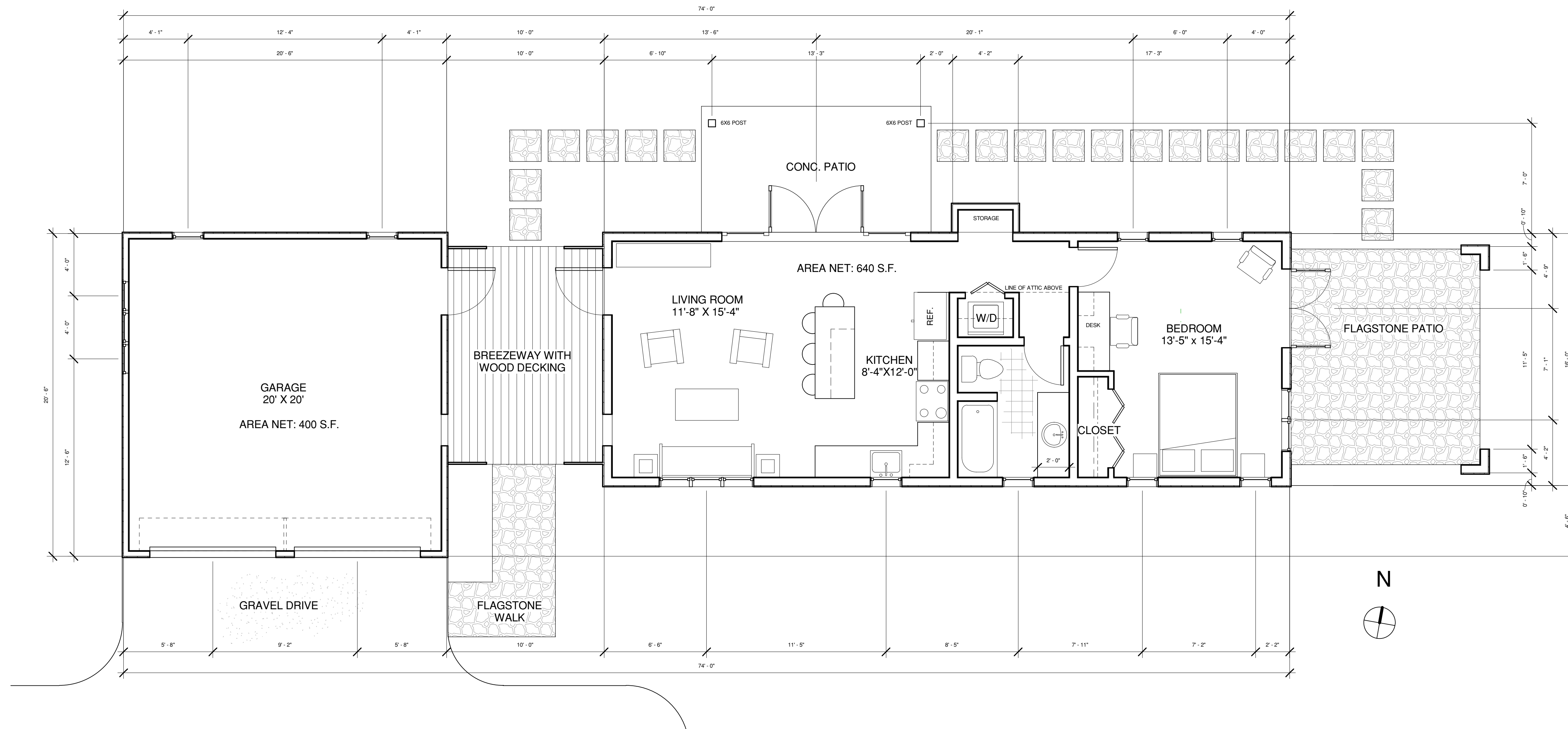
① FINISH FLOOR, VERSION 4 1/4" = 1'-0"
